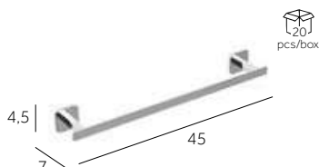
TOALLERO BARRA 45 CM
