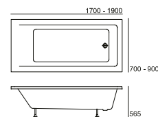
Artic 51614000 [190x90cm] 51613000 [180x80cm] 51612000 [170x75cm] 51611000 [170x70cm]
