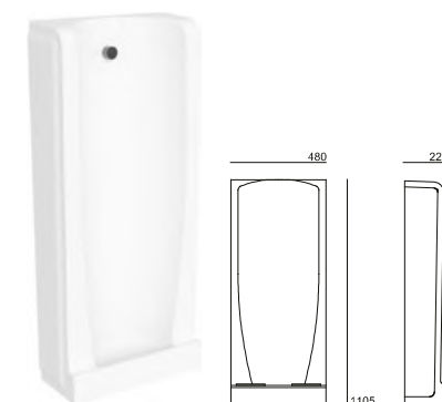
Niagara 18520XX2K [Alim. Superior . Top Inlet . Alim. Supérieure] 18521XX2K [Alim. Traseira . Back Inlet . Alim. Arrière]
