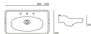
Apolo 78331XX2C [120x55x25cm] 78321XX2C [100x55x25cm] 78311XX2C [80x55x25cm]
