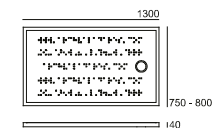
Berna 78674XX2K [130x80x4cm] 78673XX2K [130x75x4cm]
